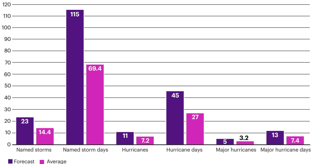
Figure 2. 2024 Hurricane prediction (forecast vs. climatology)
